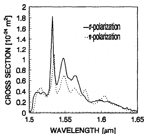
Fig. 6. Wavelength-dependent stimulated emission cross sections of Er:LiNbO 3 waveguide for \pi and \sigma polarizations.
